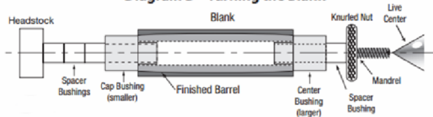
Diagram B - Turning the Blank
