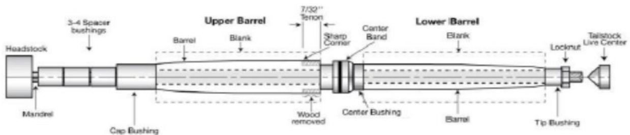
Diagram B / Turning the Blanks
