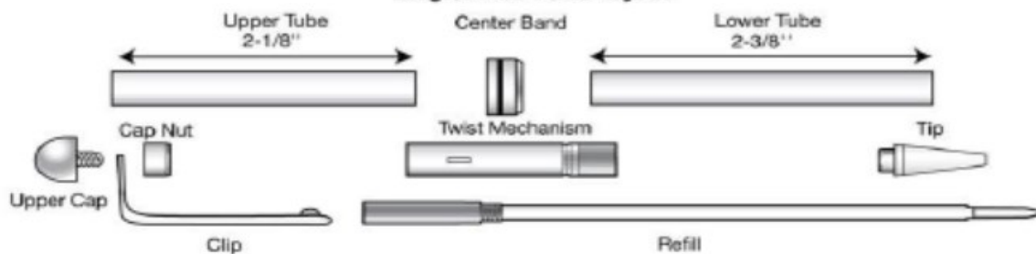
Diagram A / Parts Layout
