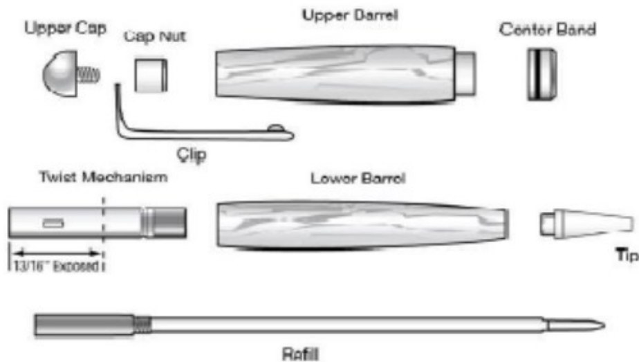
Diagram C / Assembly
