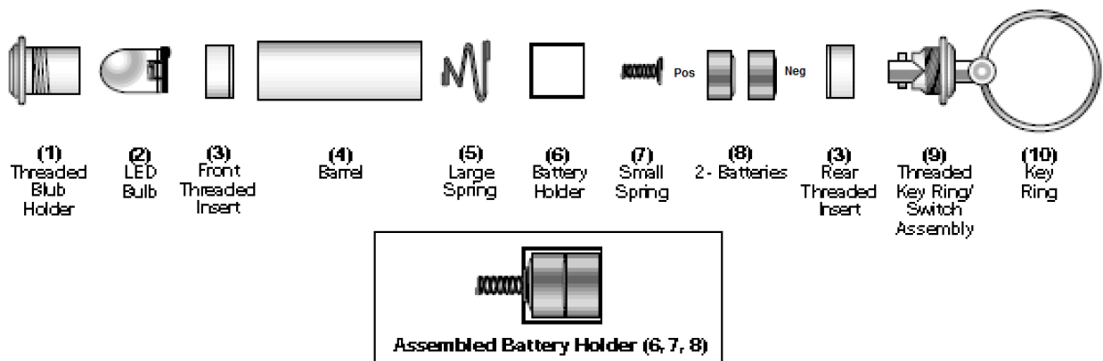
Diagram C / Penlight Assembly
