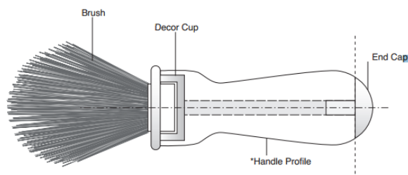
DIAGRAM B - ASSEMBLY
