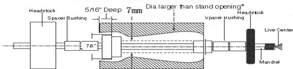
DIAGRAM A - PREPARING THE BLANK & TURNING
